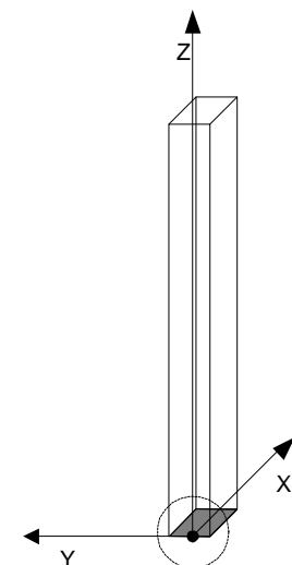
Column's local coordinate system
