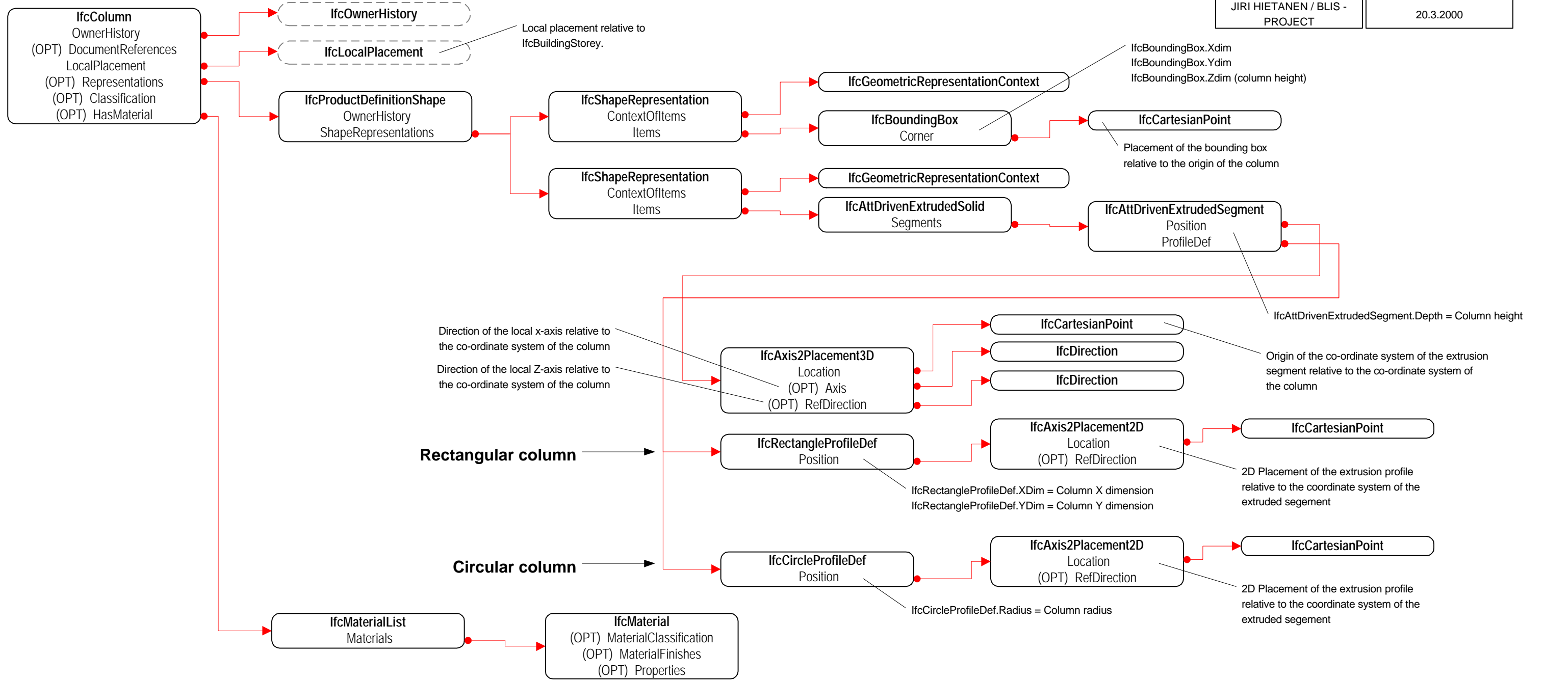
Column's local coordinate system
